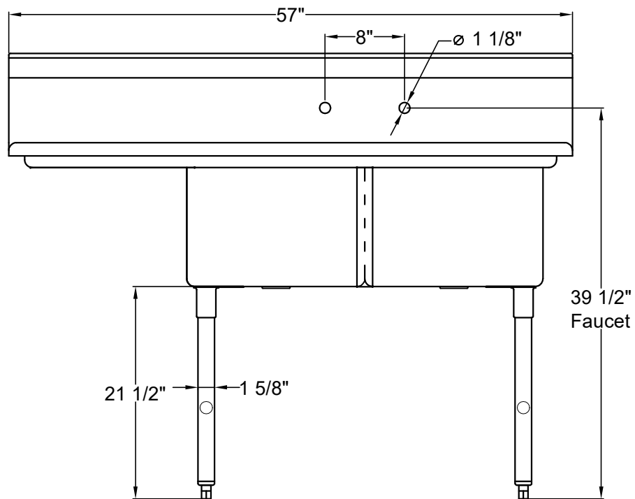
Front View
