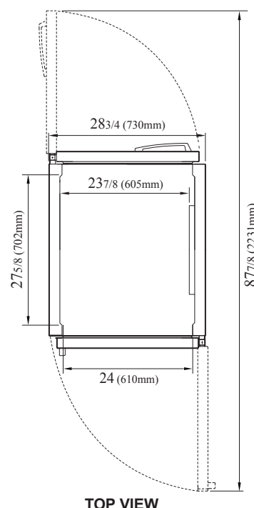
TOP VIEW
