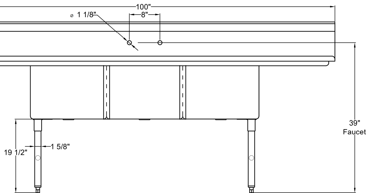
Front View
