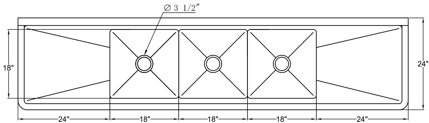
Top View
