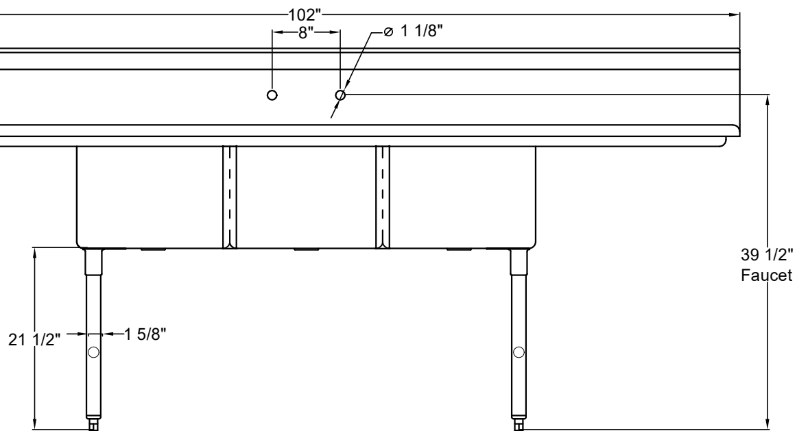
Front View
